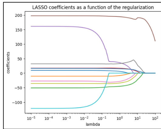
Figure 1. LASSO Coefficients
