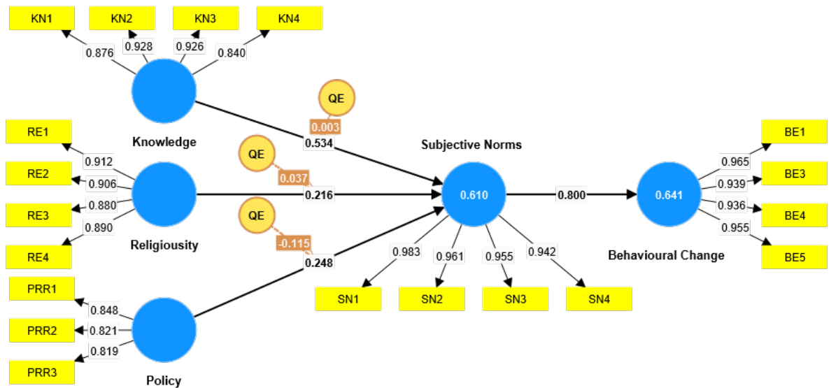
Figure 4. Test for Endogeneity – Gaussian Copula
