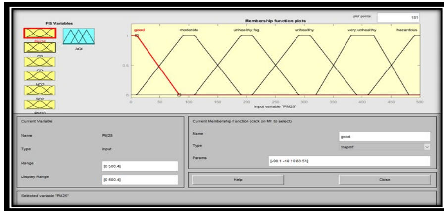
Figure 3: Membership Function of PM 2.5
