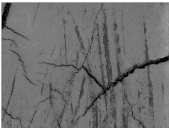
Figure 8: Morphology of the root surface debrided with curette in relation to the roughness and loss of tooth substance index (scanning electron microscope photograph, x800)
