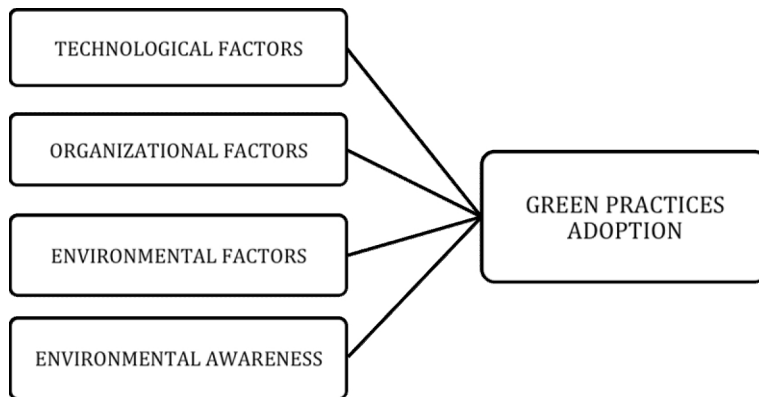
Fig. 1. Research framework
