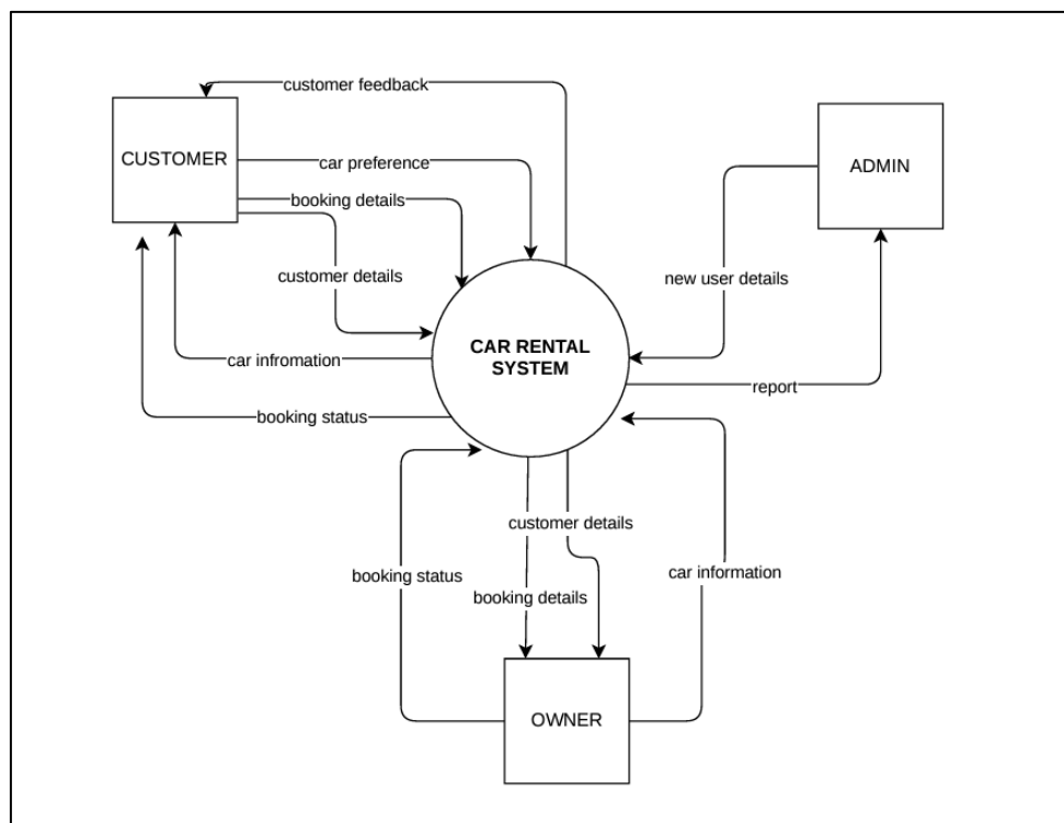
Figure 2: Context Diagram
