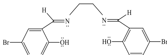
Figure 2 N,N' -Bis(5-bromosalicylidene) ethylenediamine (Brosadimine)
