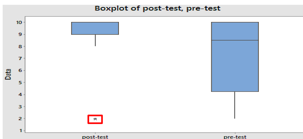
Figure 2 Boxplot
