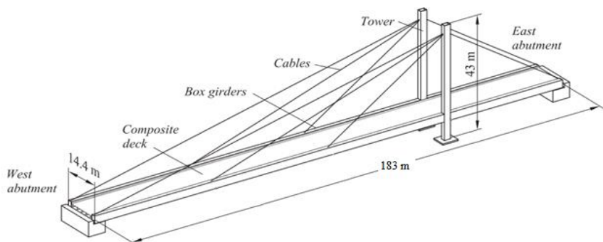
Figure 1: Detailing of Shiphaw Cable-stay Bridge
