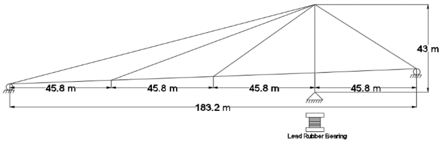
Figure 2: Bridge Model in SAP2000
