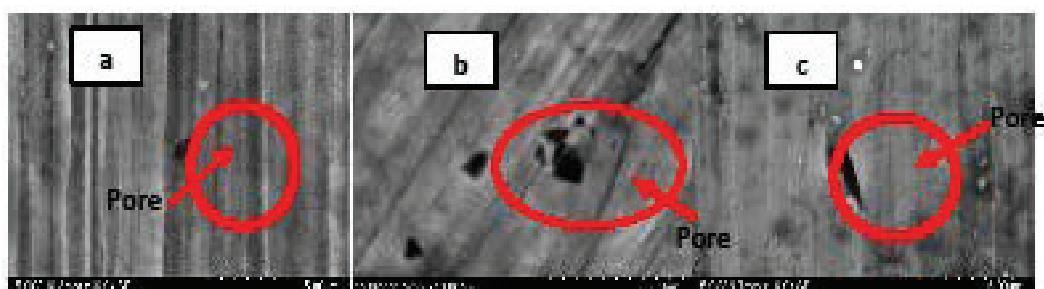
Figure 5: Microstructure After PDP in Hank's Solution for (a) Nitinol and (b) 316L SS (c) Ti-6Al-4V
