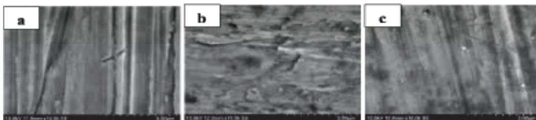
Figure 4: Microstructure of (a)316L Stainless Steel, (b) Nitinol (c)Ti-6Al-4V Before PDP in Hank' Solution
