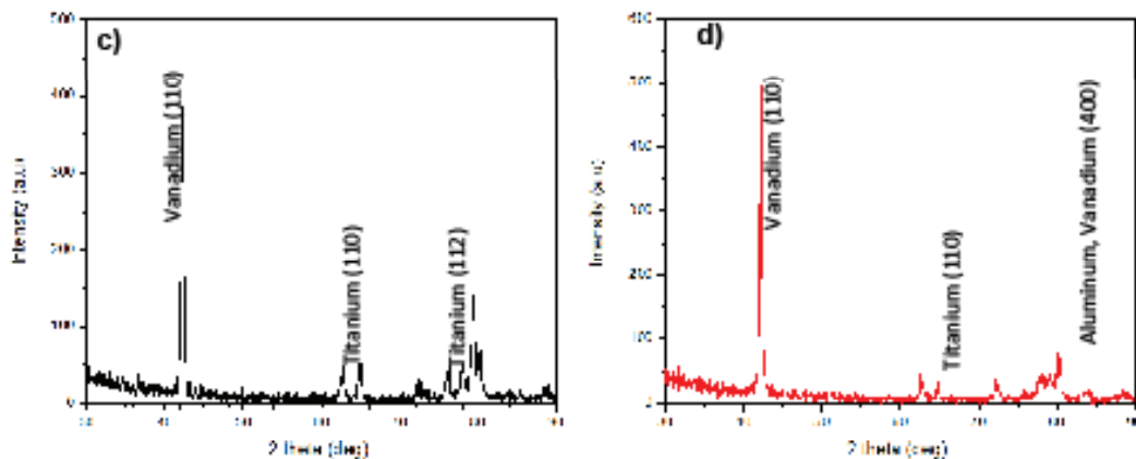
Figure 7: XRD Patterns for Ti-6Al-4V Alloys at pH Value (c) 7.4 and (d) 5.2
