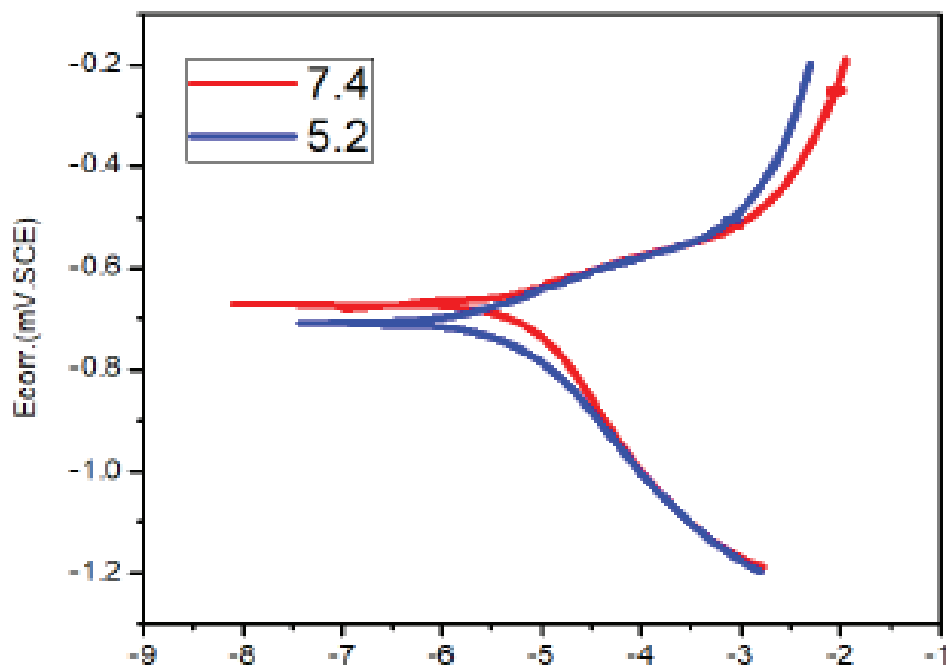
Figure 1: Potentiodynamic Polarisation Curve of 316L SS Tested in a Hank's Solution in pH 5.2 and 7.4
