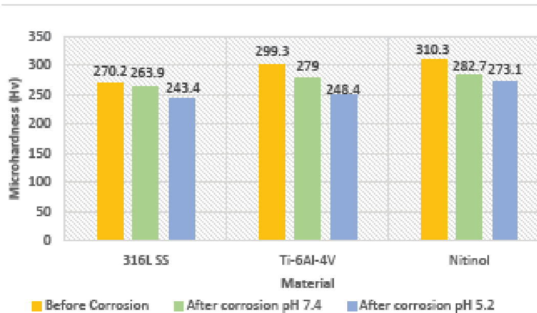
Figure 9: The Bar Chart of Microhardness under the Condition Before and After Corrosion
