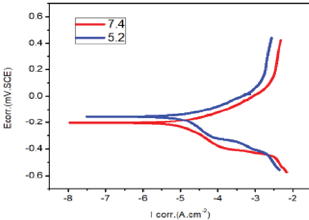
Figure 2: Potentiodynamic Polarisation Curve of Ti-6Al-4V Alloys Tested in Hank's Solution in pH 5.2 and 7.4
