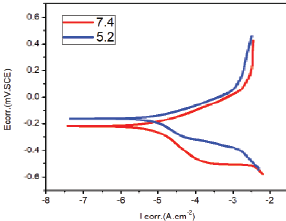
Figure 3: Potentiodynamic Polarisation Curve of Nitinol Tested in a Hank's Solution in pH 5.2 and 7.4
