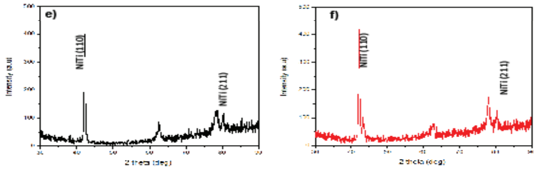
Figure 8: XRD Patterns for Nitinol at pH Value (e) 7.4 and (f) 5.2
