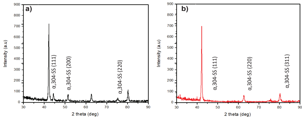
Figure 6: XRD Patterns for 316L SS at pH Value (a) 7.4 and (b) 5.2
