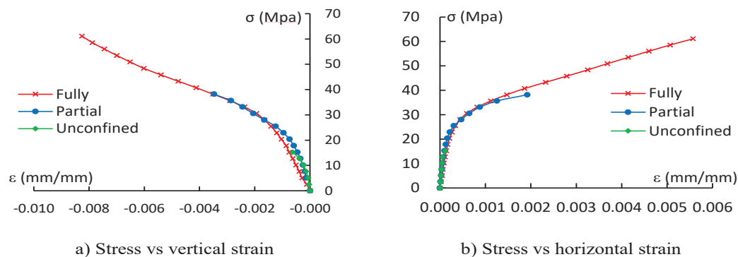
Figure 4: Stress-Strain Relationship
