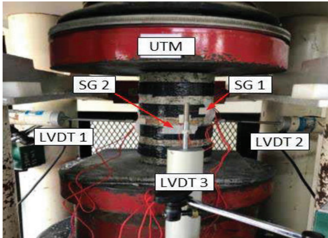
Figure 2: Experimental Setup
