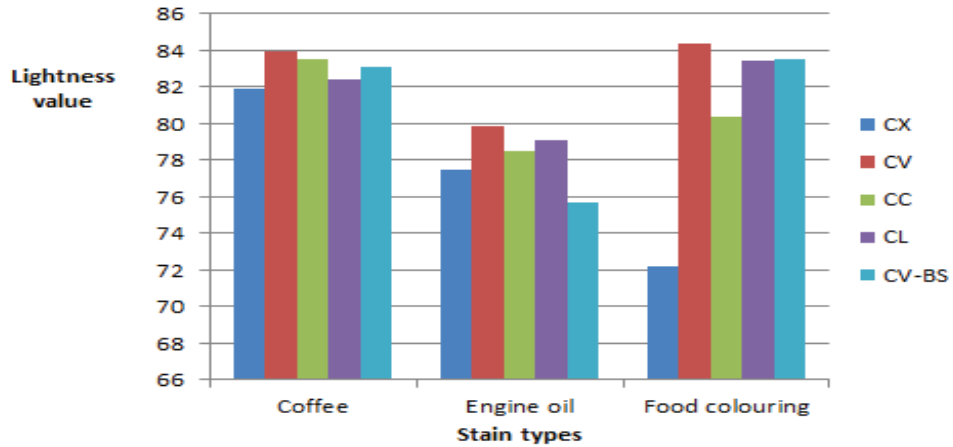
Figure 6: Lightness Value for Cotton
