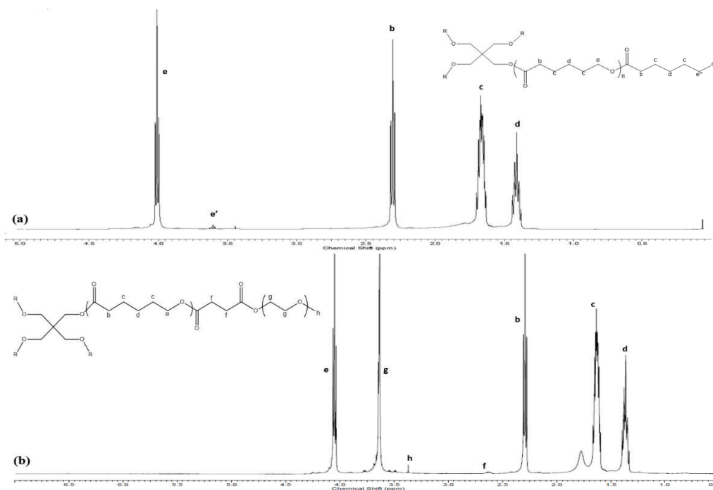
Figure 2: ^1\text{H-NMR} Spectra of a) 4Star PCL and b) 4Star PCL-PEG
