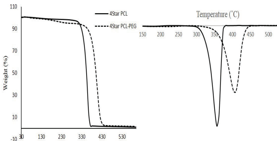
Figure 3: TGA and DTG Thermograms Curve for 4Star PCL and 4Star PCL-PEG
