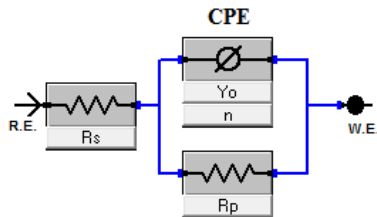
Figure 3: Equivalent circuit fit for the Nyquist plots
