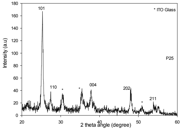
Figure 1: XRD spectrum of TiO 2 film after annealing at 450°C for 60 minutes
