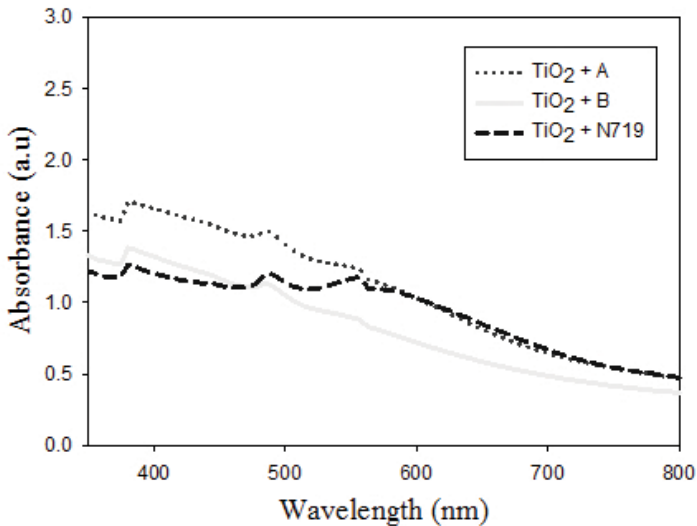
Figure 3: Absorption spectra of \text{TiO}_2 film after immersion with the dyes for 24 hours
