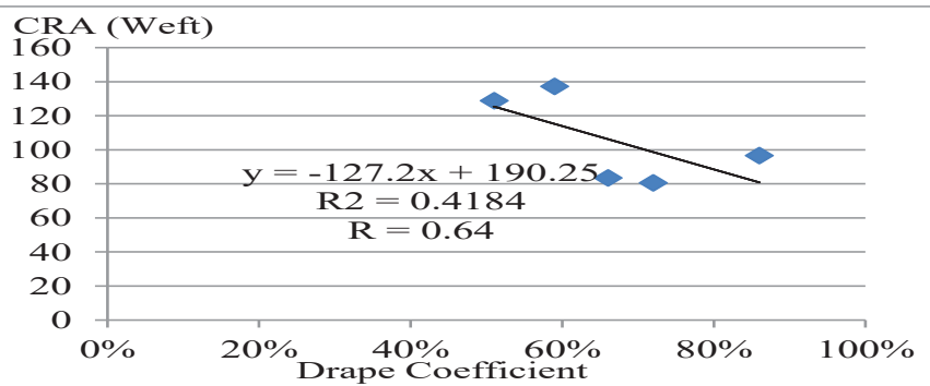
Figure 16: The relationship between the crease angle recovery (weft) and the drapability of the fabric
