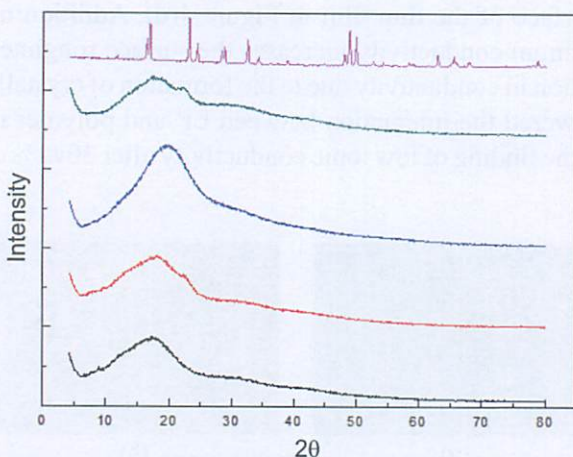
Figure 4: XRD Pattern for MG30-PEMA, Pure \text{LiCF}_3\text{SO}_3 and MG30-PEMA with Selected \text{LiCF}_3\text{SO}_3 Salt Composition
