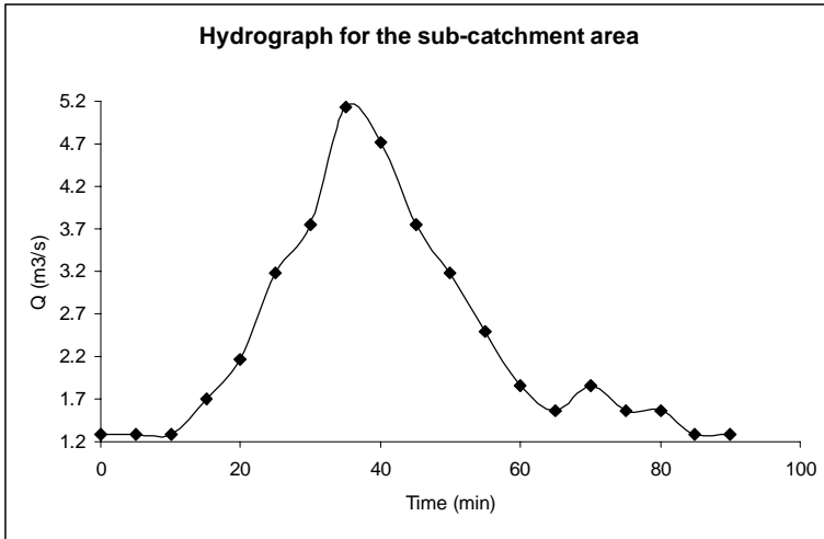
Figure 4: Hydrograph Discharge
